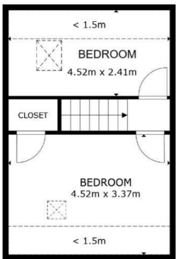
FLOOR 4
